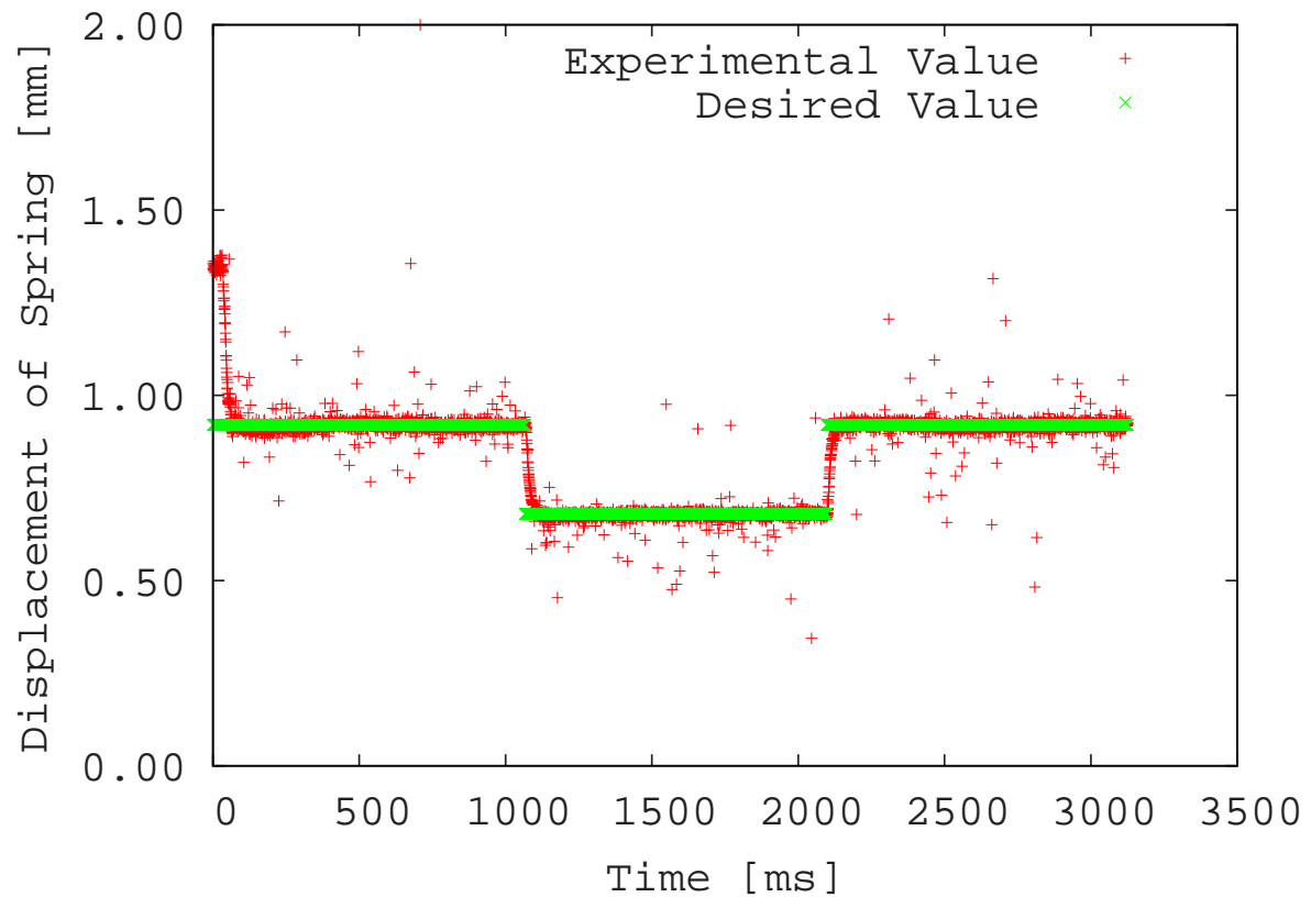
Fig. 12 Displacement of Spring (for Changing Desired Load)
